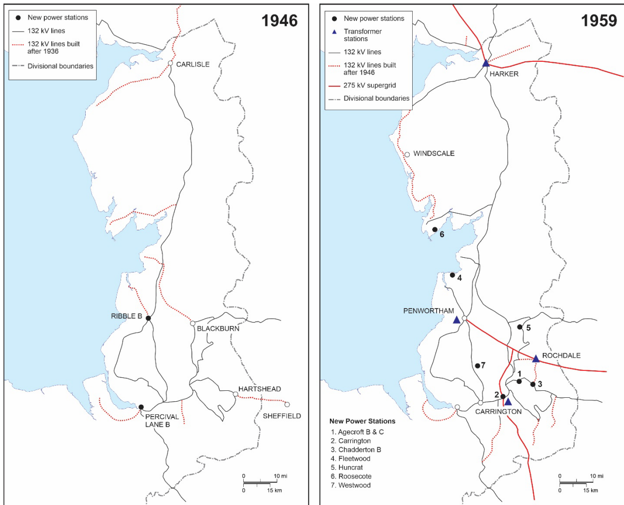
Figure 6 DEVELOPMENT OF THE NATIONAL GRID 1946 and 1959.
